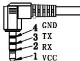
Figure 2: Pin Assignment
